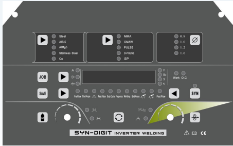
Control panel: material, method, wire diameter, program memory, gas check, wire inching, trigger, and pulse setup.
