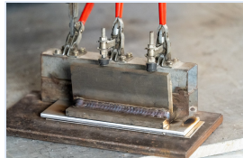
MIG-500XW Stainless steel · 10 mm SINGLE PULSE
