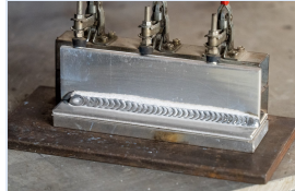
MFL-200 Aluminum · 1.5 mm SINGLE PULSE
