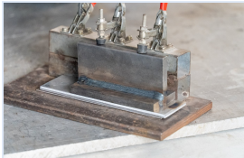
MIG-500XW Carbon steel · 10 mm SINGLE PULSE
