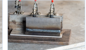
MIG-500 Stainless steel · 10 mm DOUBLE PULSE
