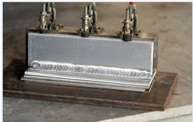
MIG-500 Aluminum · 5 mm SINGLE PULSE
